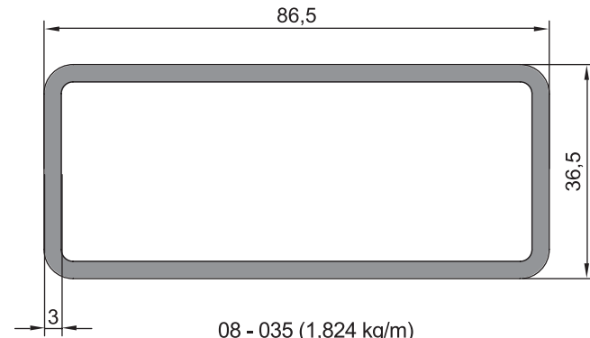
08 - 035 (1,824 kg/m)
