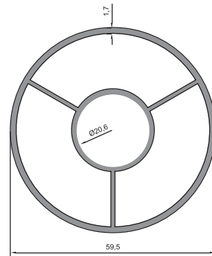
08 - 048 (1,317 kg/m)
