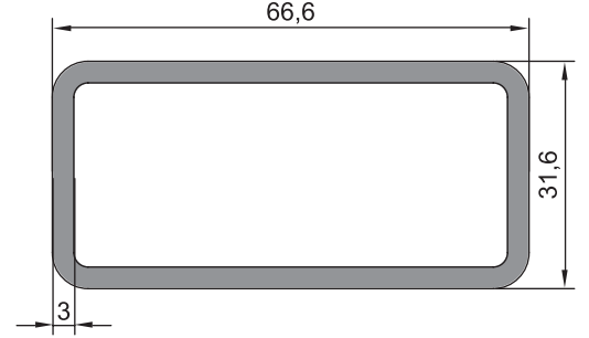
08 - 036 (1,450 kg/m)
