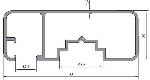
08 - 055 (1,114 kg/m)
