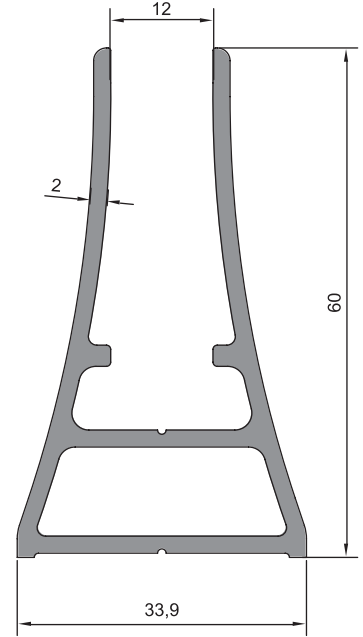
08 - 071 (1,005 kg/m)
