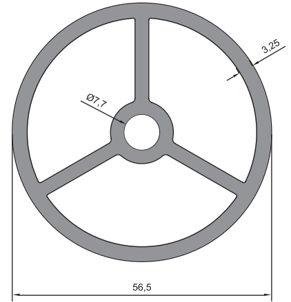
08 - 074 (2,192 kg/m)
